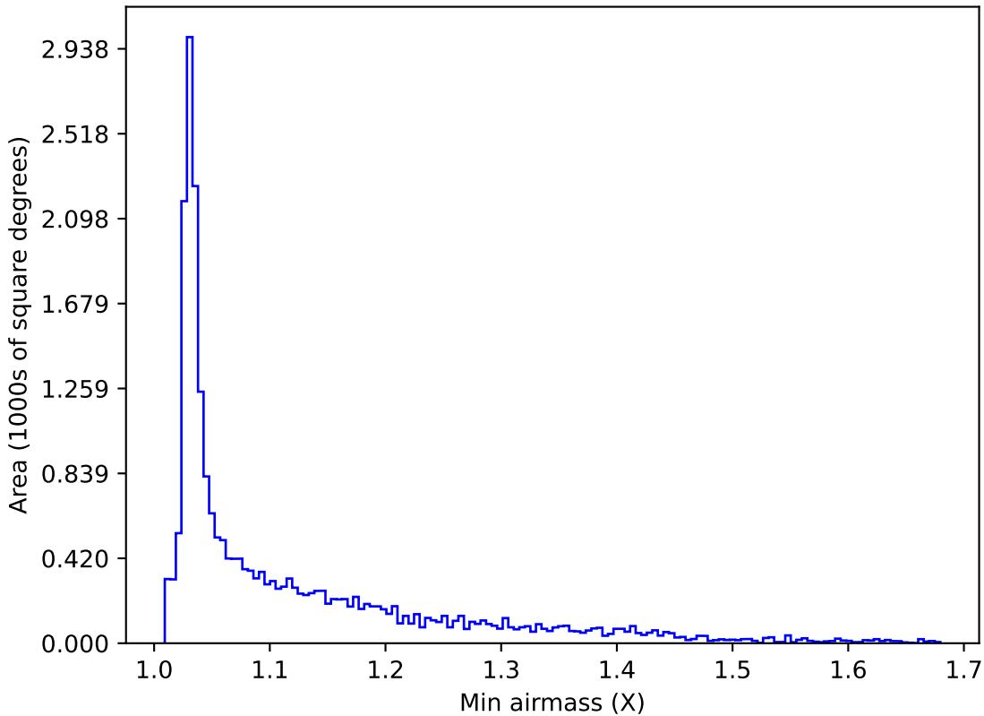
too_elab_r64_d2_ugrizy_v3.4_10yrs All sky y band: Min airmass
