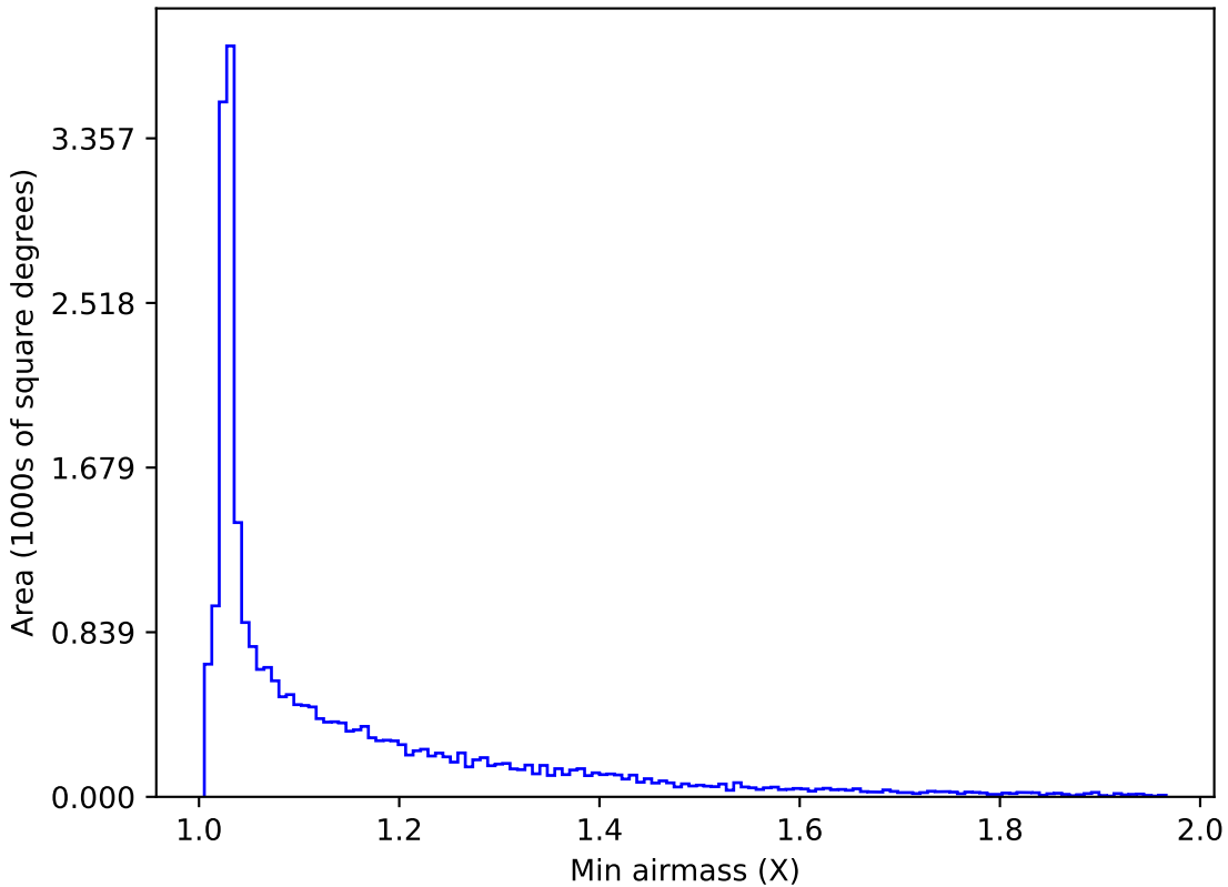
too_elab_r64_d2_ugrizy_v3.4_10yrs All sky i band: Min airmass
