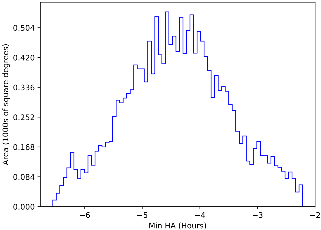
too_elab_r64_d2_ugrizy_v3.4_10yrs WFD z band: Min HA
