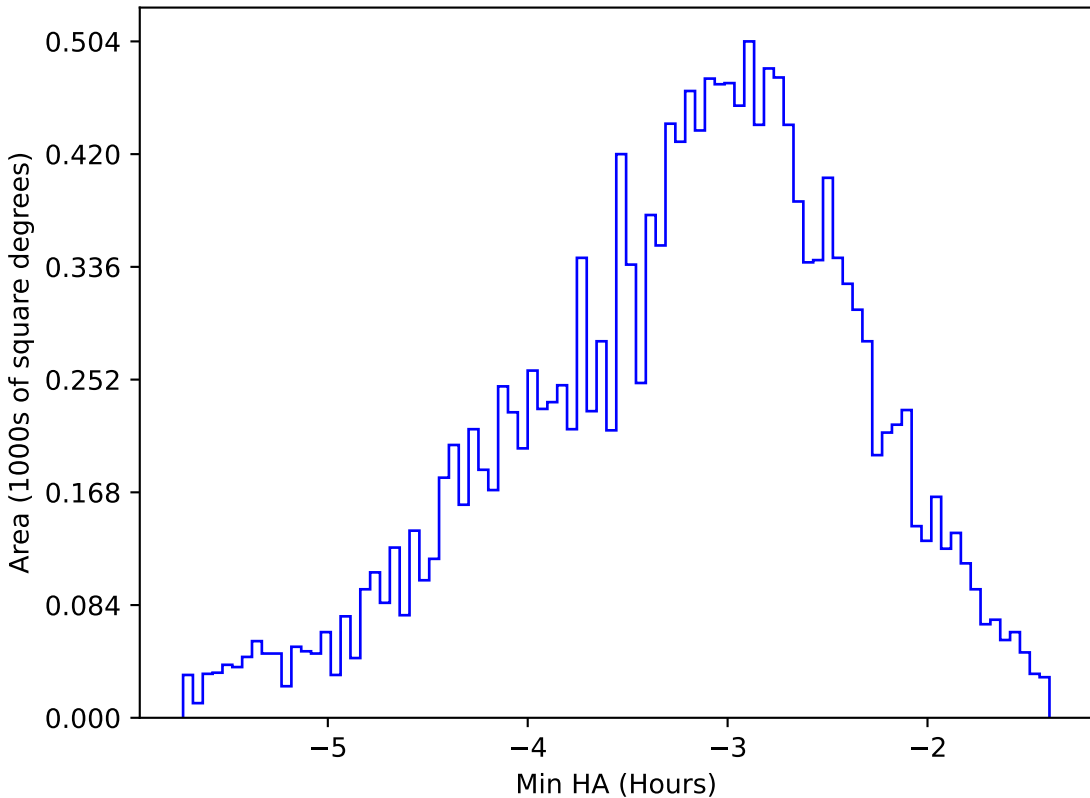
too_elab_r64_d2_ugrizy_v3.4_10yrs WFD u band: Min HA
