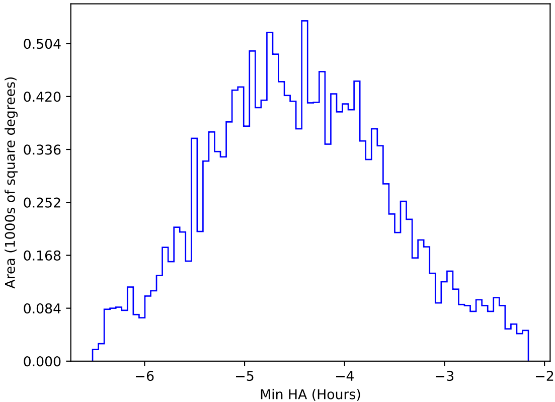
too_elab_r64_d2_ugrizy_v3.4_10yrs WFD i band: Min HA
