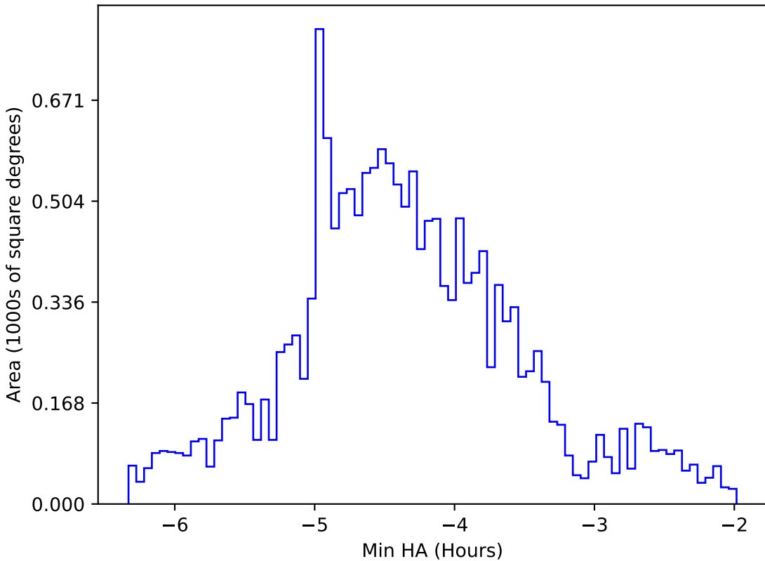
too_elab_r64_d2_ugrizy_v3.4_10yrs WFD g band: Min HA
