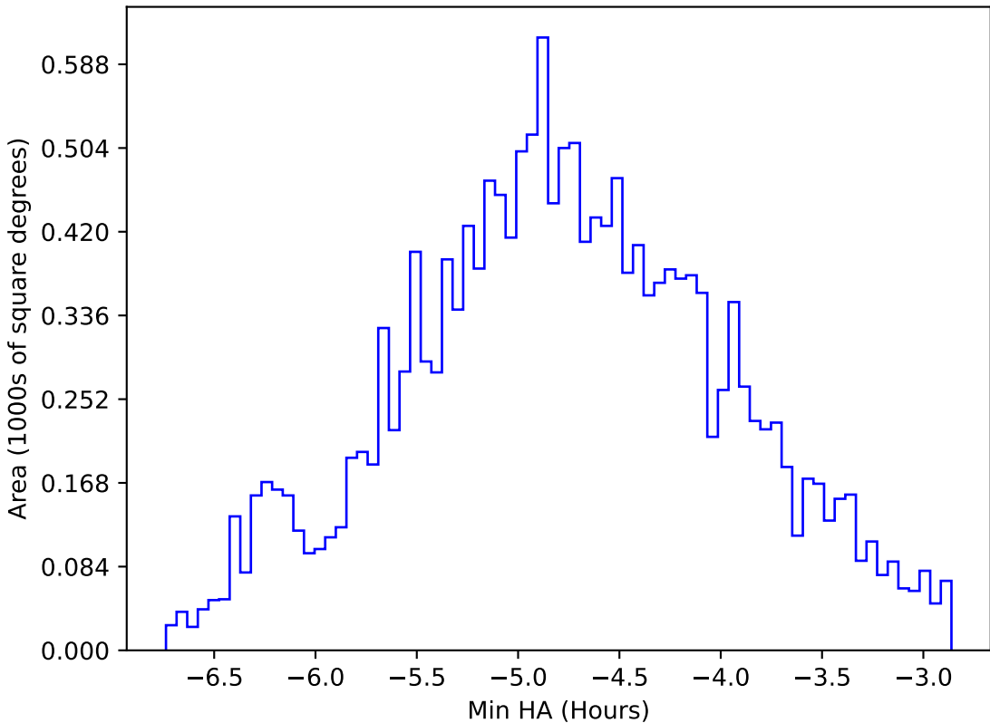
too_elab_r64_d2_ugrizy_v3.4_10yrs WFD all bands: Min HA
