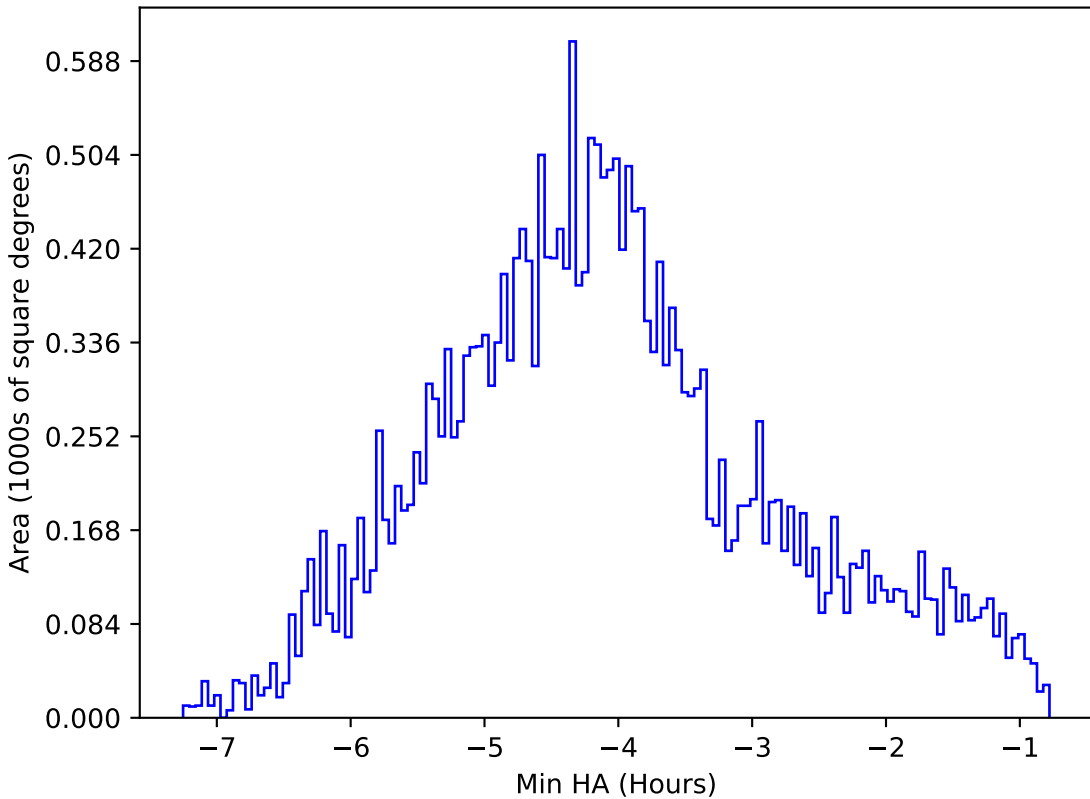
too_elab_r64_d2_ugrizy_v3.4_10yrs All sky z band: Min HA
