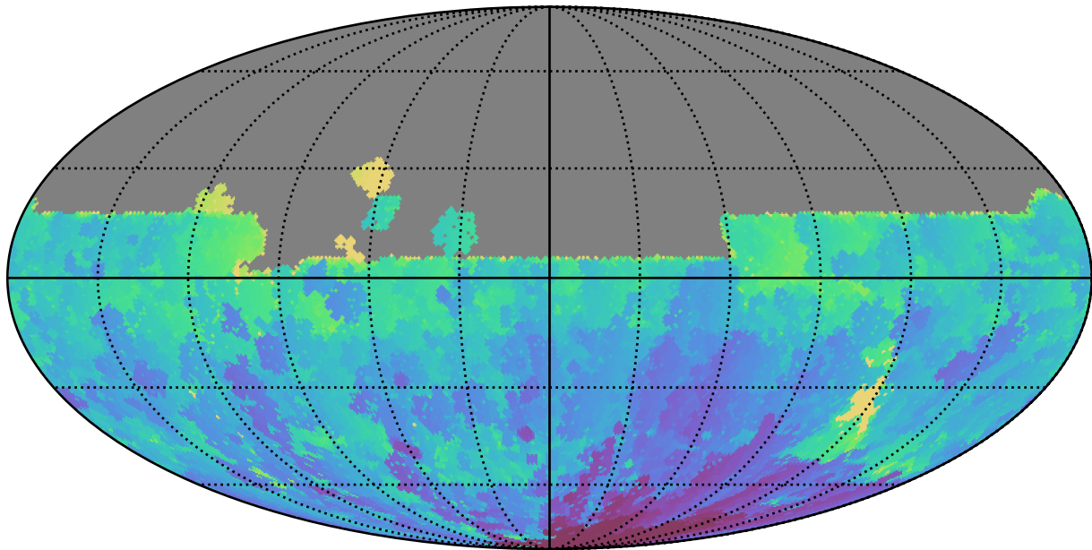
too_elab_r64_d2_ugrizy_v3.4_10yrs All sky u band: Min HA
