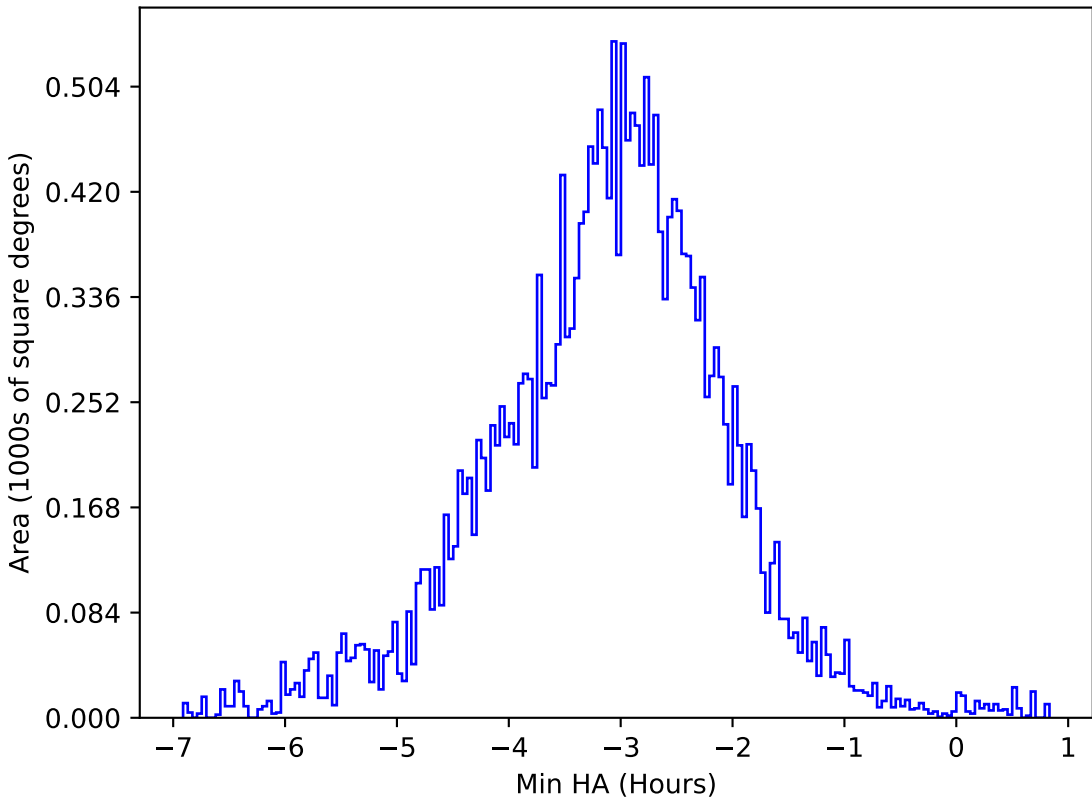
too_elab_r64_d2_ugrizy_v3.4_10yrs All sky u band: Min HA
