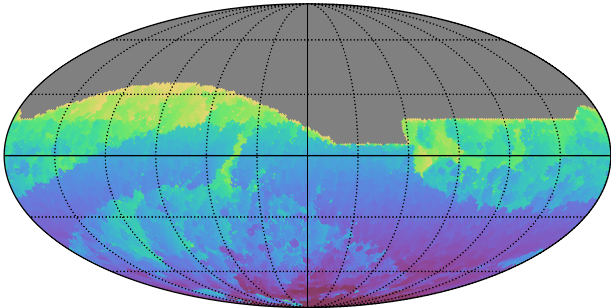
too_elab_r64_d2_ugrizy_v3.4_10yrs All sky r band: Min HA
