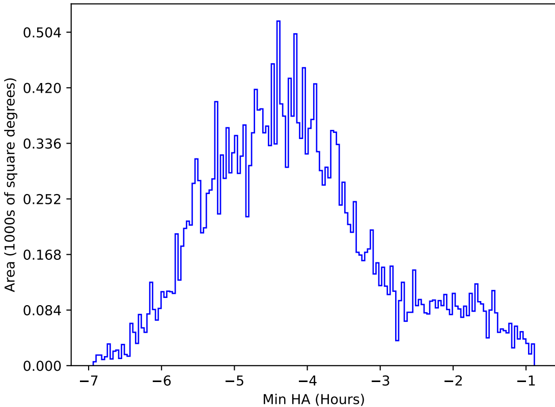
too_elab_r64_d2_ugrizy_v3.4_10yrs All sky r band: Min HA
