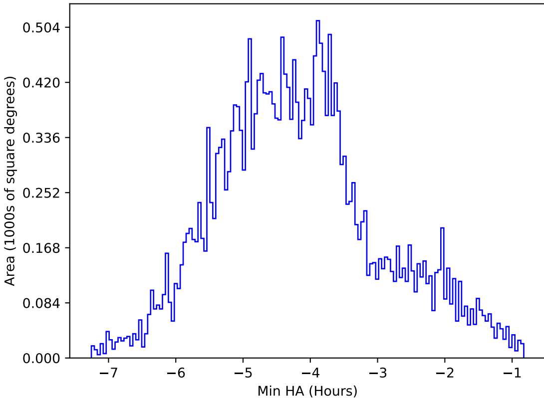
too_elab_r64_d2_ugrizy_v3.4_10yrs All sky i band: Min HA
