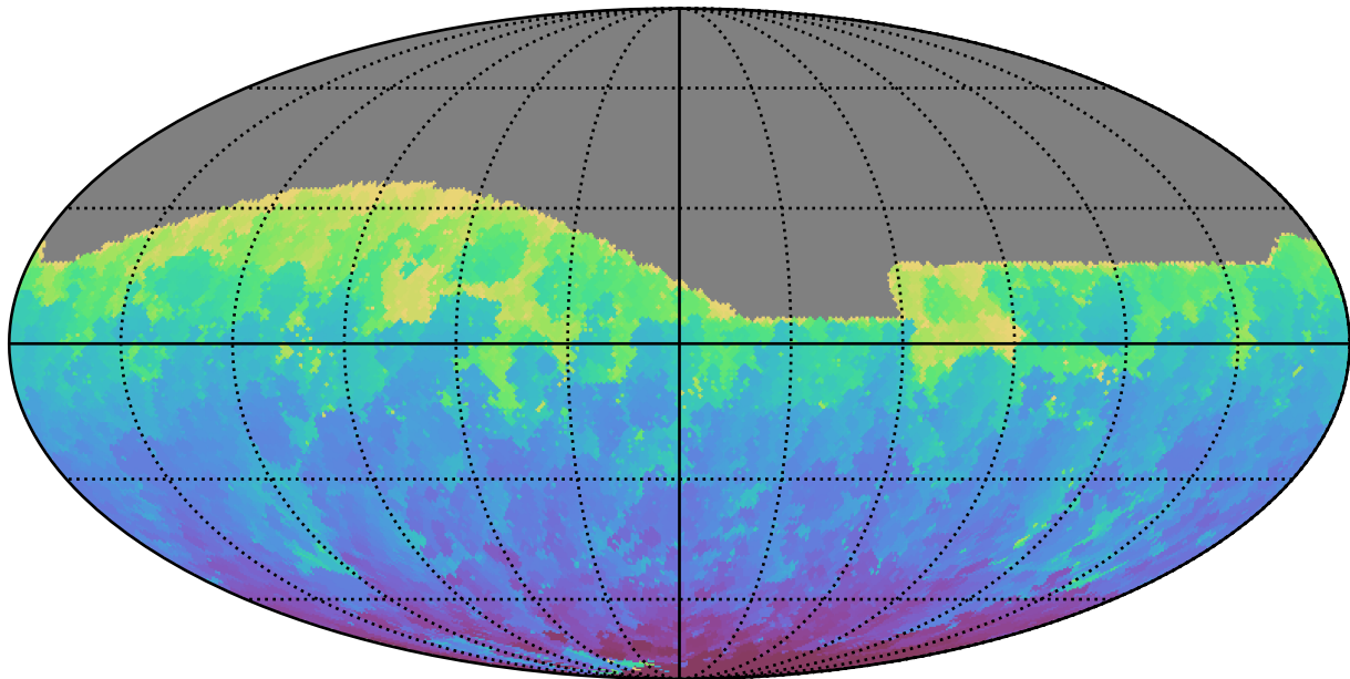
too_elab_r64_d2_ugrizy_v3.4_10yrs All sky g band: Min HA
