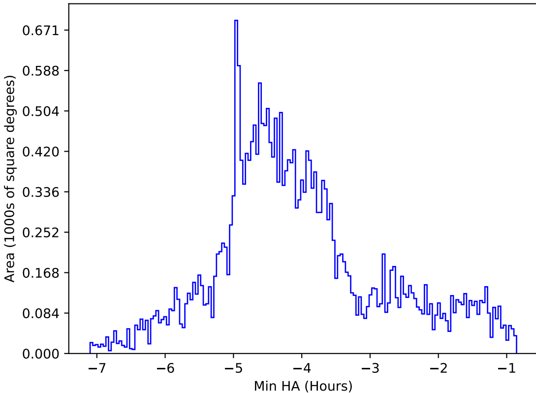
too_elab_r64_d2_ugrizy_v3.4_10yrs All sky g band: Min HA
