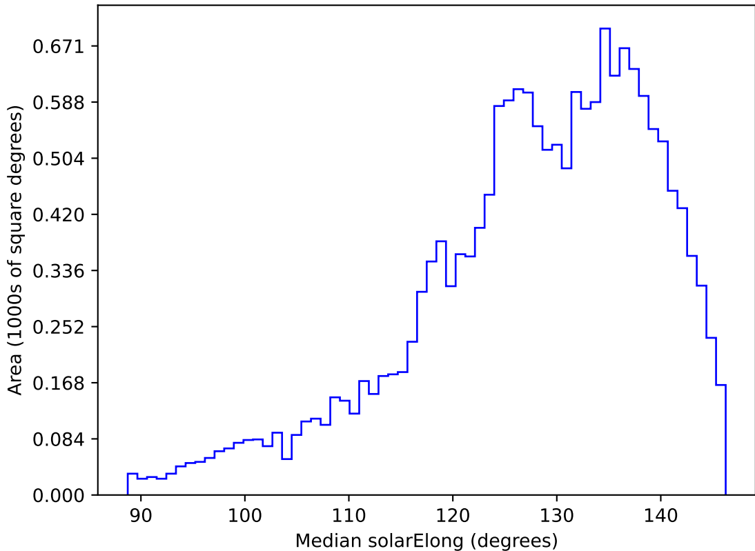
too_elab_r64_d2_ugrizy_v3.4_10yrs WFD z band: Median solarElong
