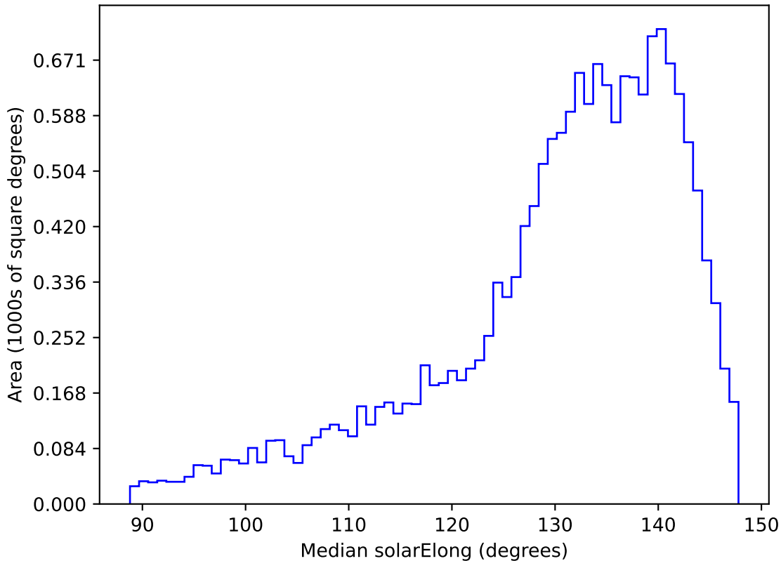
too_elab_r64_d2_ugrizy_v3.4_10yrs WFD y band: Median solarElong
