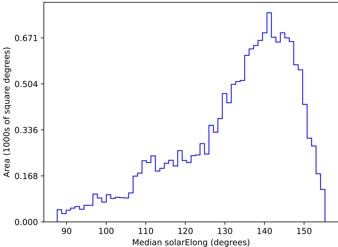
too_elab_r64_d2_ugrizy_v3.4_10yrs WFD u band: Median solarElong
