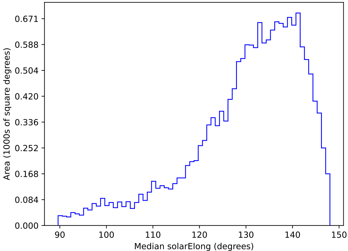
too_elab_r64_d2_ugrizy_v3.4_10yrs WFD r band: Median solarElong
