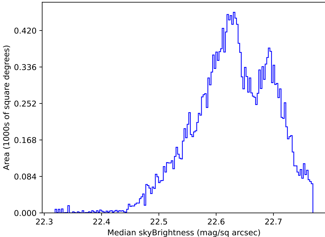
too_elab_r64_d2_ugrizy_v3.4_10yrs Yr 1 u band: Median skyBrightness
