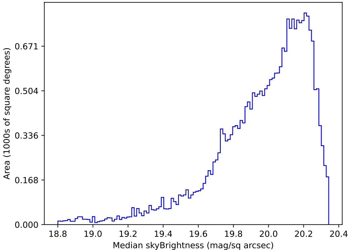
too_elab_r64_d2_ugrizy_v3.4_10yrs Yr 1 i band: Median skyBrightness
