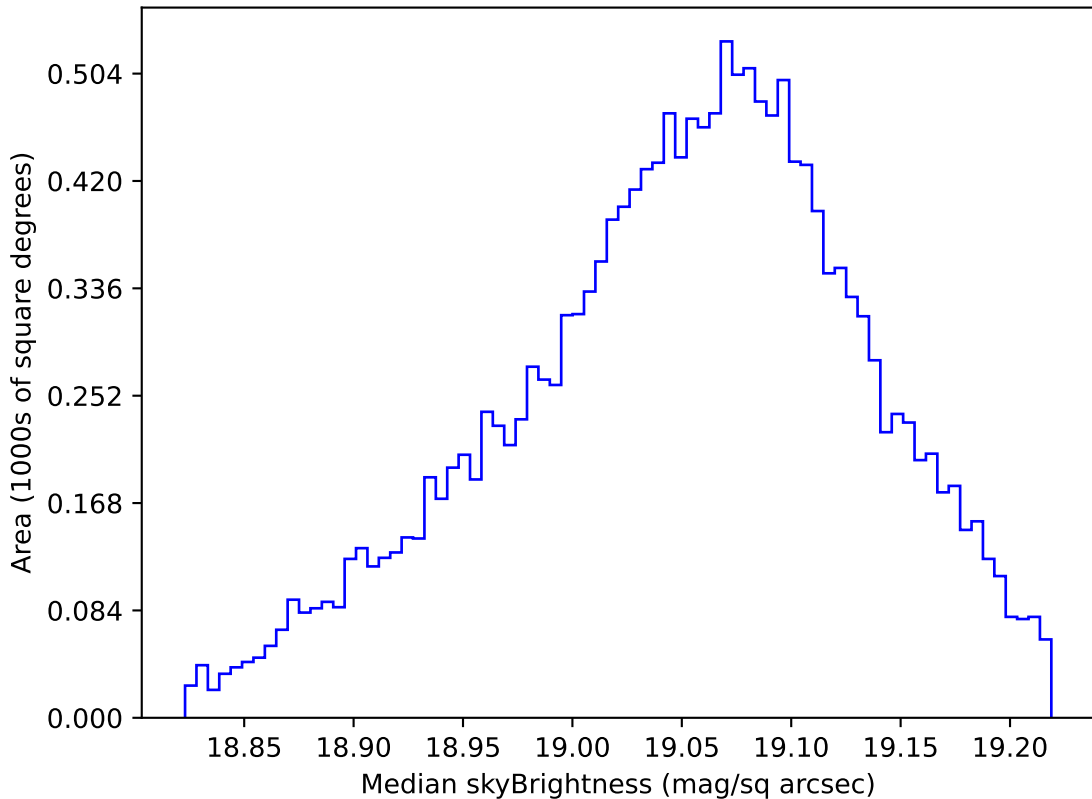
too_elab_r64_d2_ugrizy_v3.4_10yrs WFD z band: Median skyBrightness
