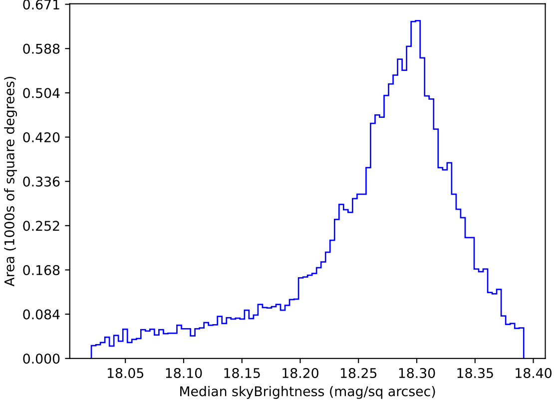
too_elab_r64_d2_ugrizy_v3.4_10yrs WFD y band: Median skyBrightness
