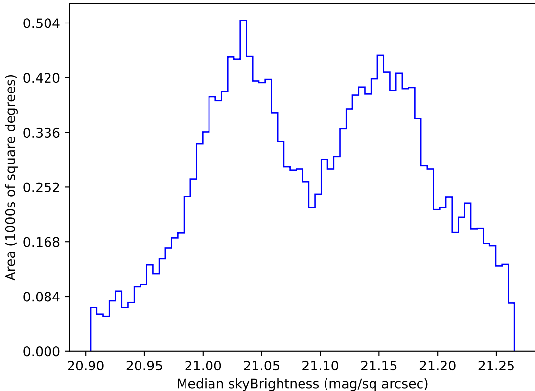
too_elab_r64_d2_ugrizy_v3.4_10yrs WFD r band: Median skyBrightness
