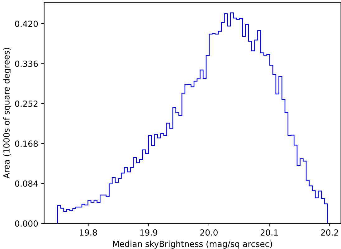
too_elab_r64_d2_ugrizy_v3.4_10yrs WFD i band: Median skyBrightness
