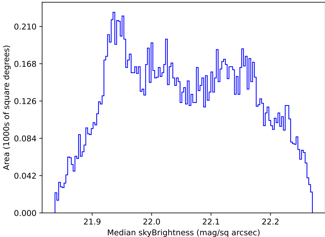
too_elab_r64_d2_ugrizy_v3.4_10yrs WFD g band: Median skyBrightness
