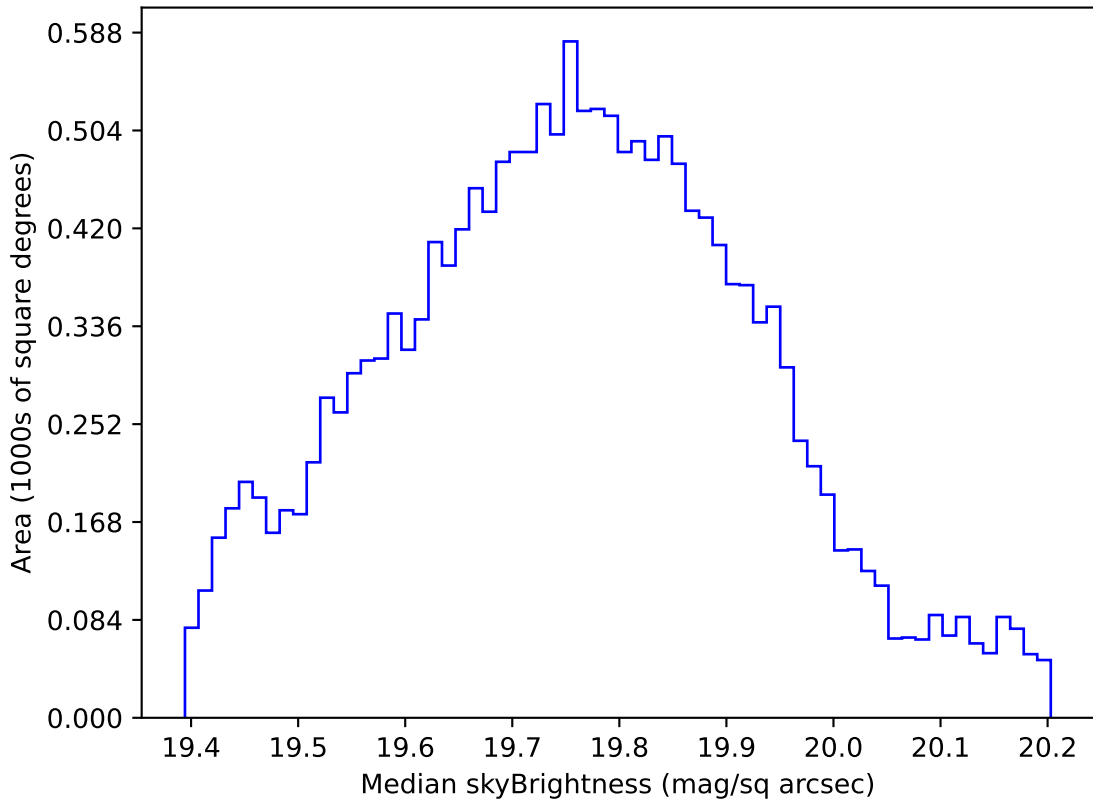
too_elab_r64_d2_ugrizy_v3.4_10yrs WFD all bands: Median skyBrightness
