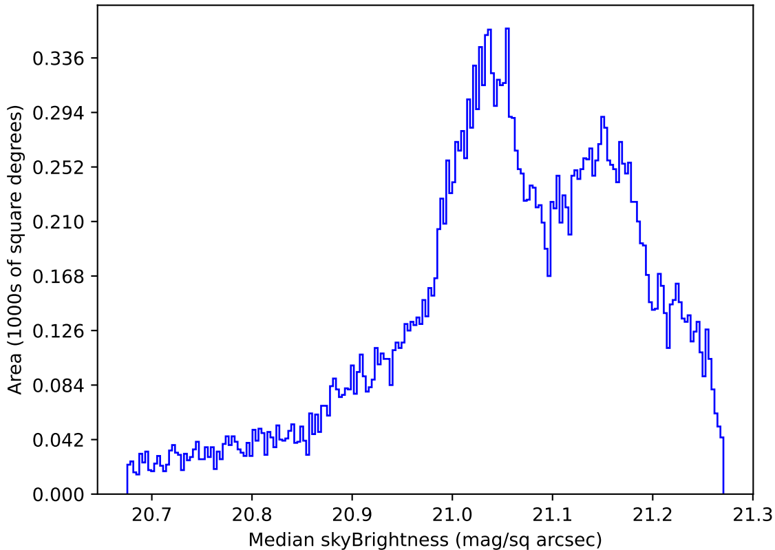
too_elab_r64_d2_ugrizy_v3.4_10yrs All sky r band: Median skyBrightness
