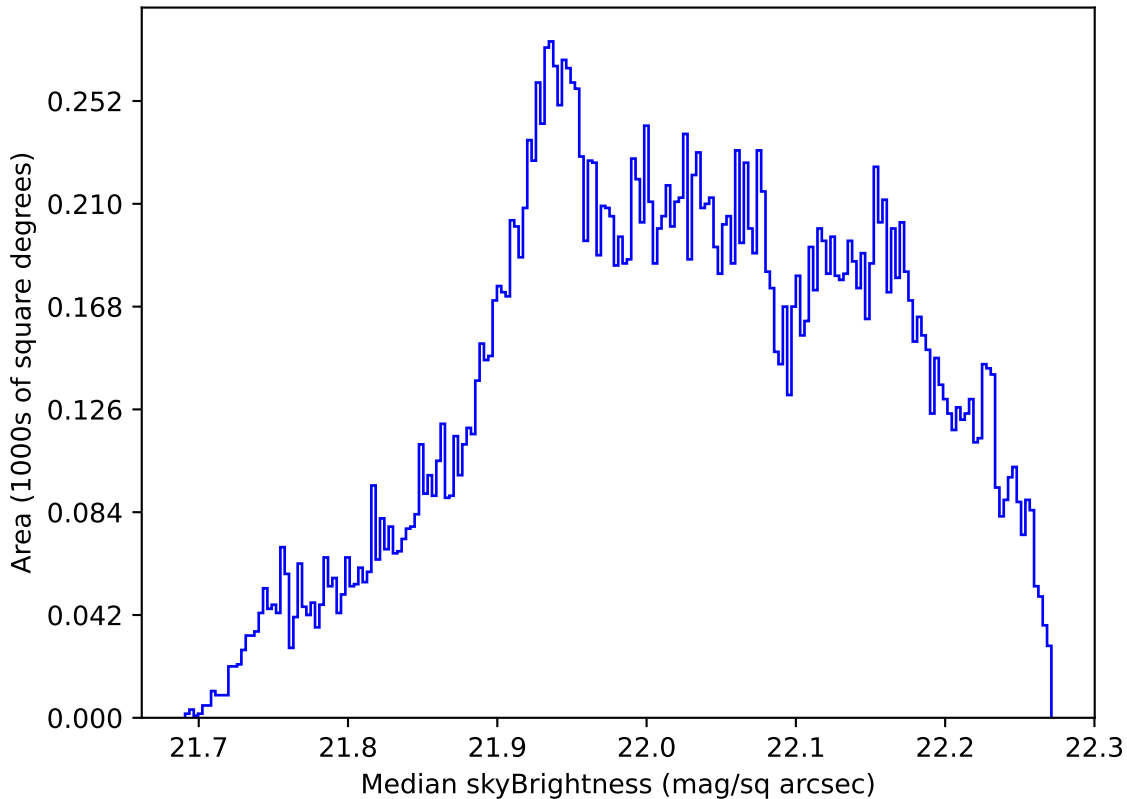
too_elab_r64_d2_ugrizy_v3.4_10yrs All sky g band: Median skyBrightness
