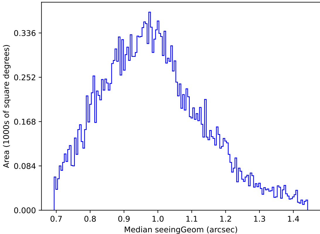
too_elab_r64_d2_ugrizy_v3.4_10yrs Yr 1 u band: Median seeingGeom
