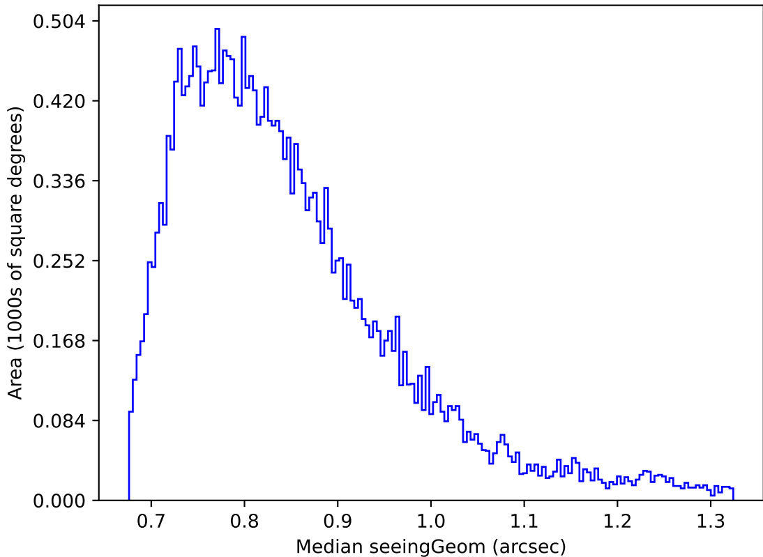
too_elab_r64_d2_ugrizy_v3.4_10yrs Yr 1 i band: Median seeingGeom
