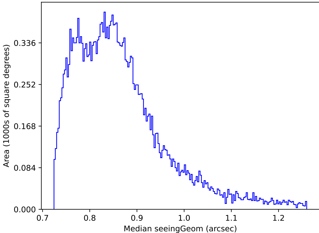
too_elab_r64_d2_ugrizy_v3.4_10yrs Yr 1 all bands: Median seeingGeom
