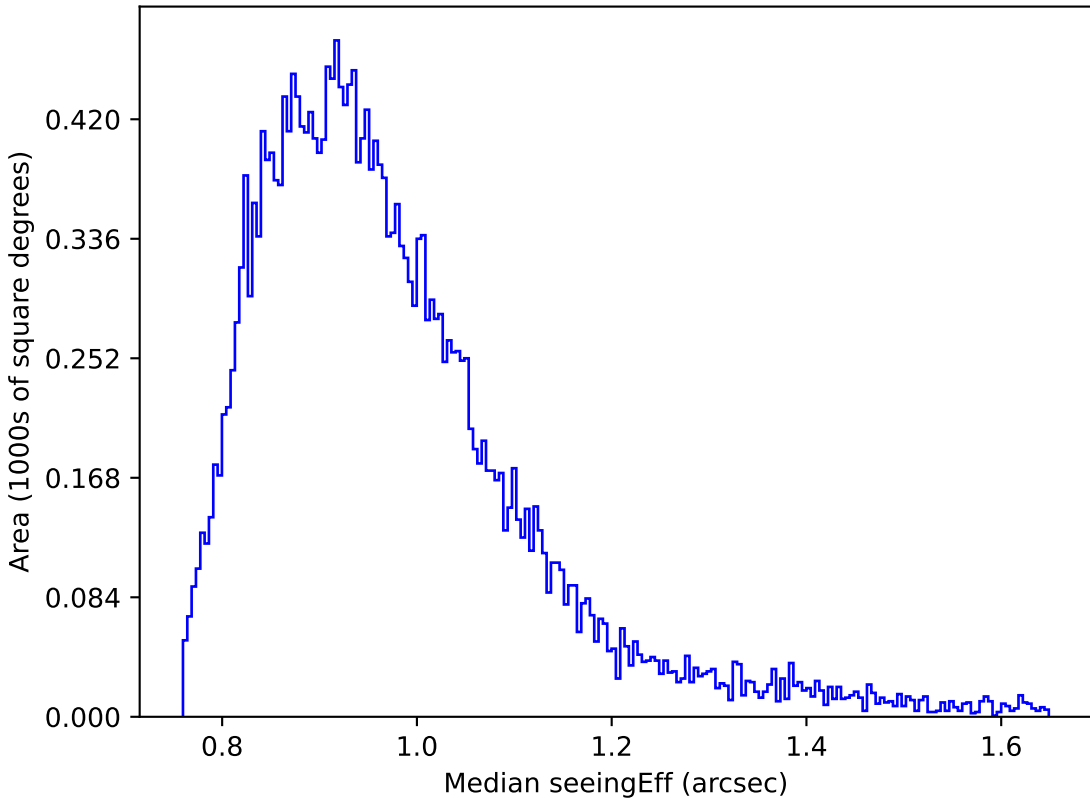
too_elab_r64_d2_ugrizy_v3.4_10yrs Yr 1 z band: Median seeingEff
