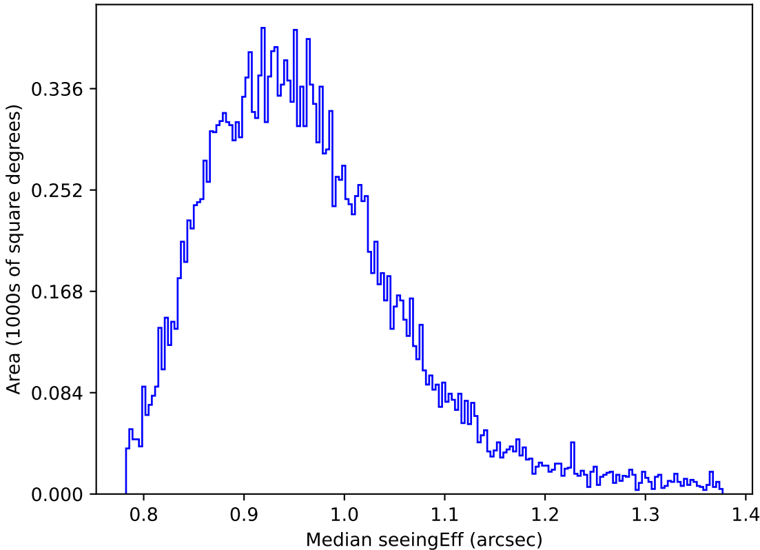
too_elab_r64_d2_ugrizy_v3.4_10yrs Yr 1 y band: Median seeingEff
