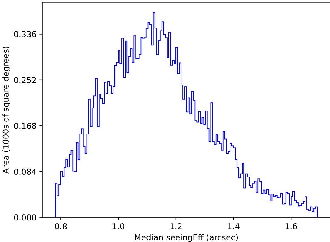
too_elab_r64_d2_ugrizy_v3.4_10yrs Yr 1 u band: Median seeingEff
