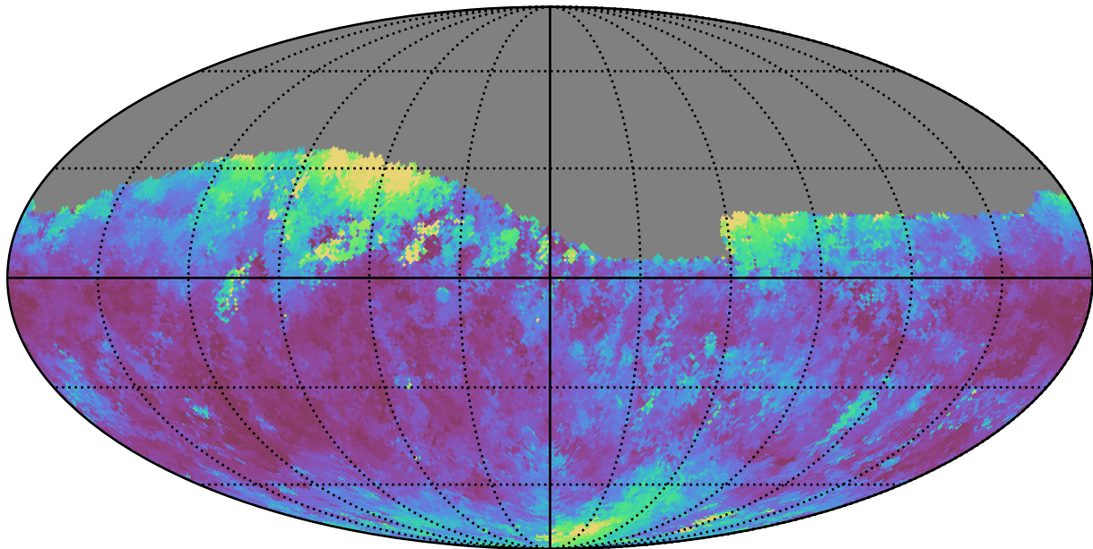
too_elab_r64_d2_ugrizy_v3.4_10yrs Yr 1 r band: Median seeingEff
