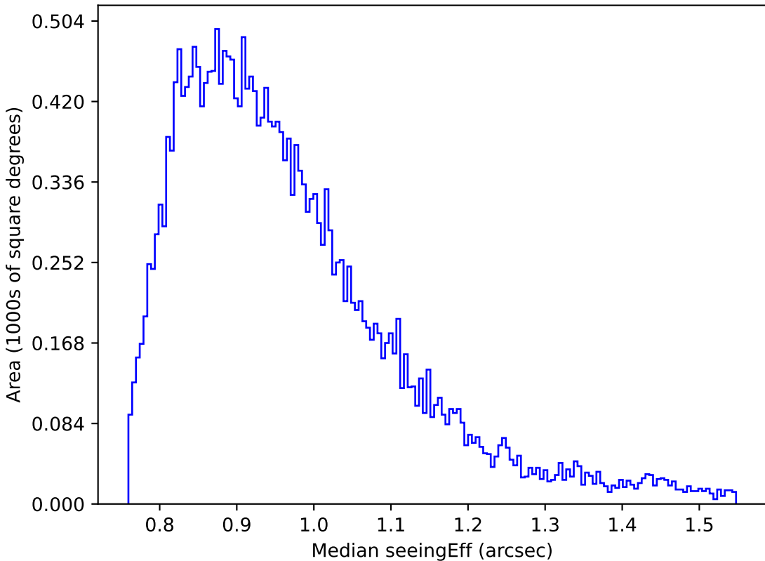
too_elab_r64_d2_ugrizy_v3.4_10yrs Yr 1 i band: Median seeingEff
