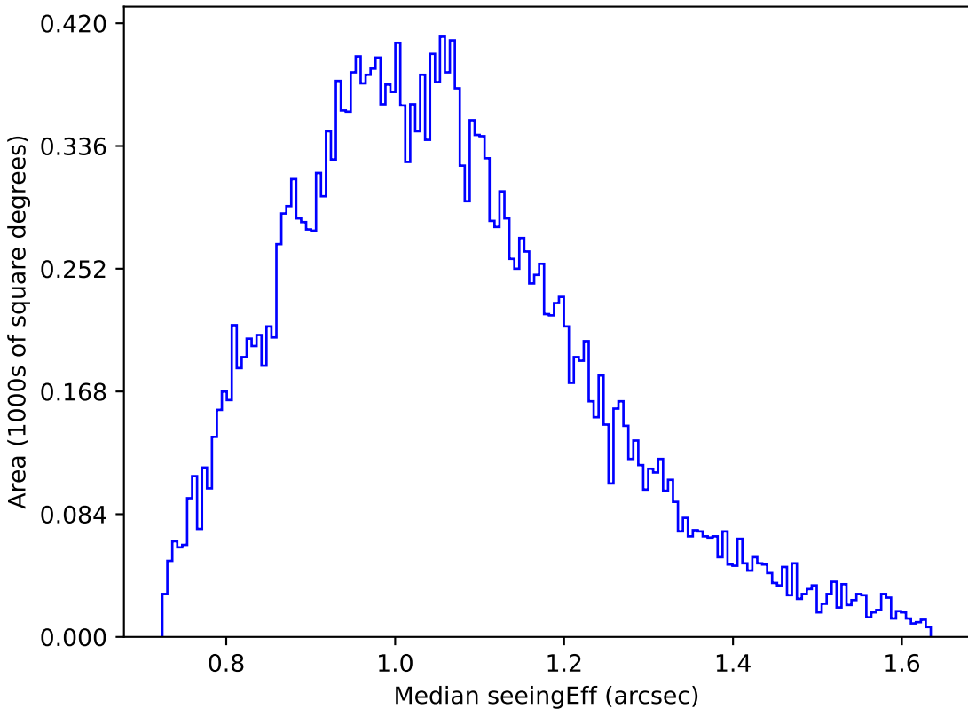
too_elab_r64_d2_ugrizy_v3.4_10yrs Yr 1 g band: Median seeingEff
