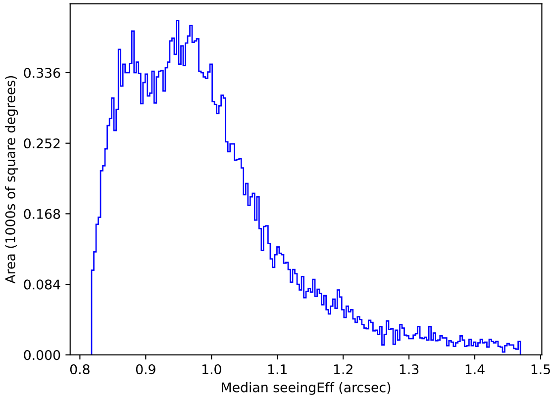
too_elab_r64_d2_ugrizy_v3.4_10yrs Yr 1 all bands: Median seeingEff
