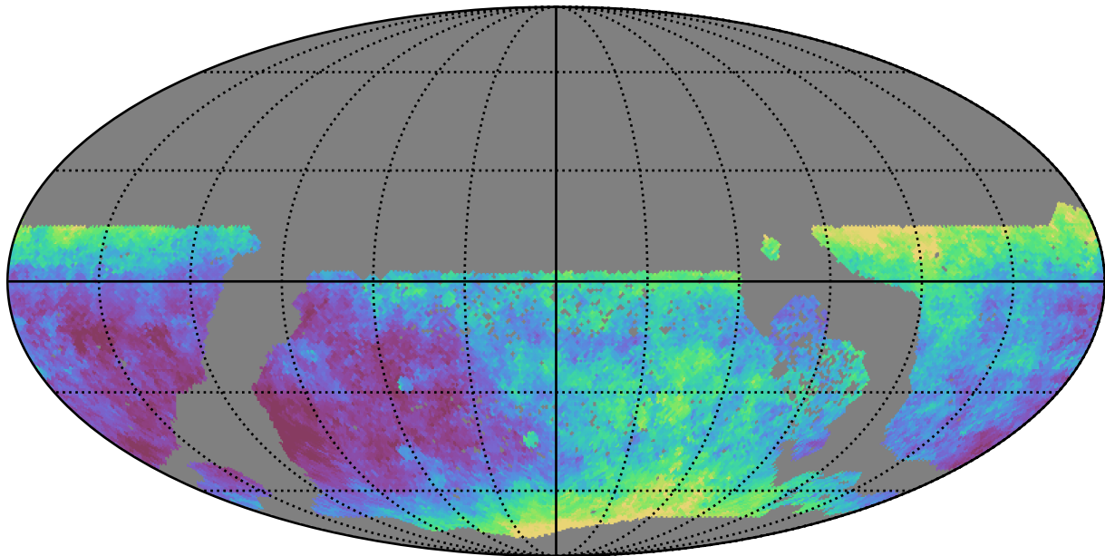
too_elab_r64_d2_ugrizy_v3.4_10yrs WFD z band: Median seeingEff
