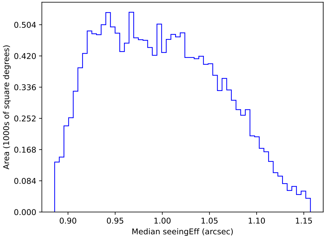
too_elab_r64_d2_ugrizy_v3.4_10yrs WFD y band: Median seeingEff
