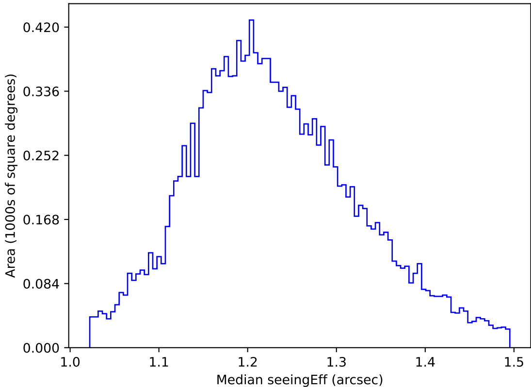
too_elab_r64_d2_ugrizy_v3.4_10yrs WFD u band: Median seeingEff
