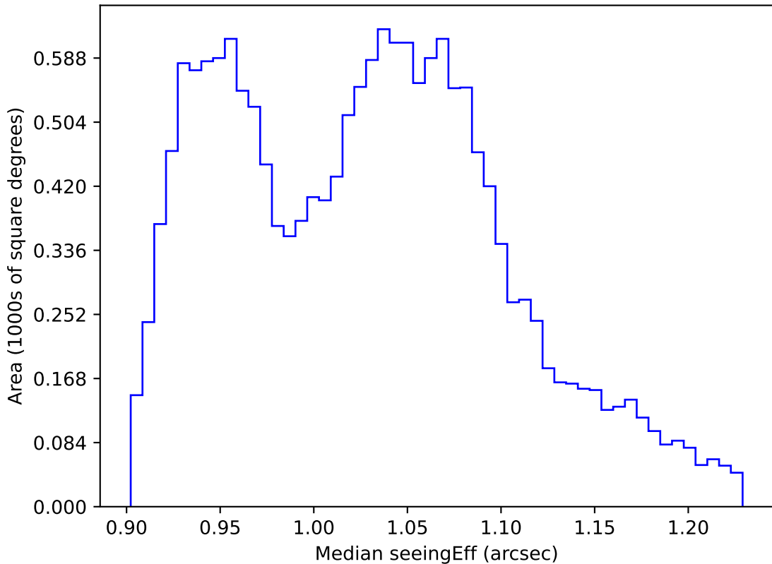
too_elab_r64_d2_ugrizy_v3.4_10yrs WFD all bands: Median seeingEff
