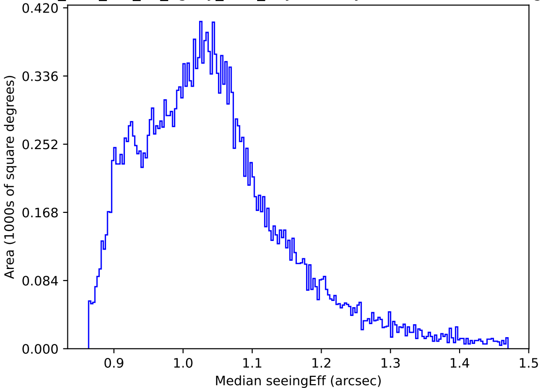
too_elab_r64_d2_ugrizy_v3.4_10yrs All sky z band: Median seeingEff
