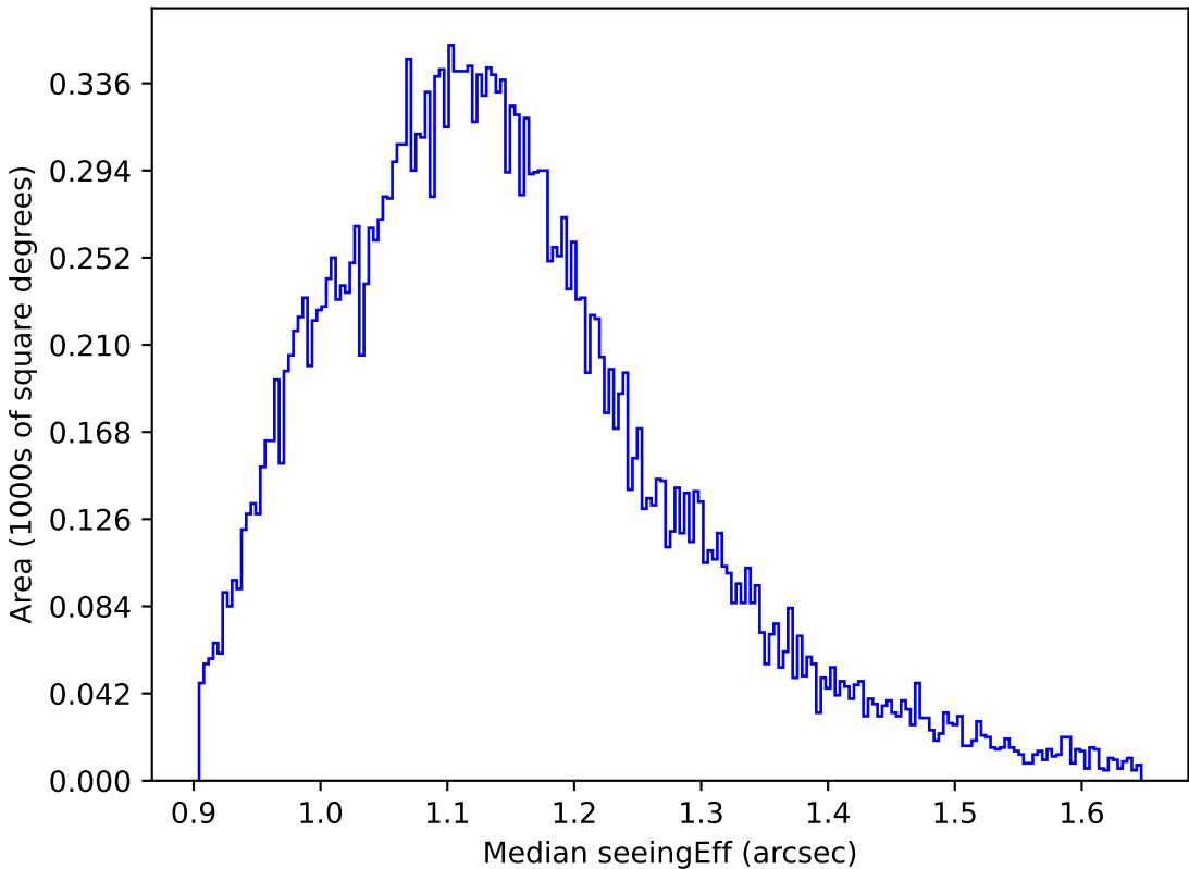
too_elab_r64_d2_ugrizy_v3.4_10yrs All sky g band: Median seeingEff
