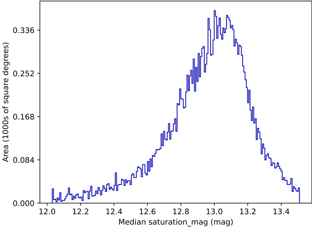
too_elab_r64_d2_ugrizy_v3.4_10yrs All sky u band: Median saturation_mag
