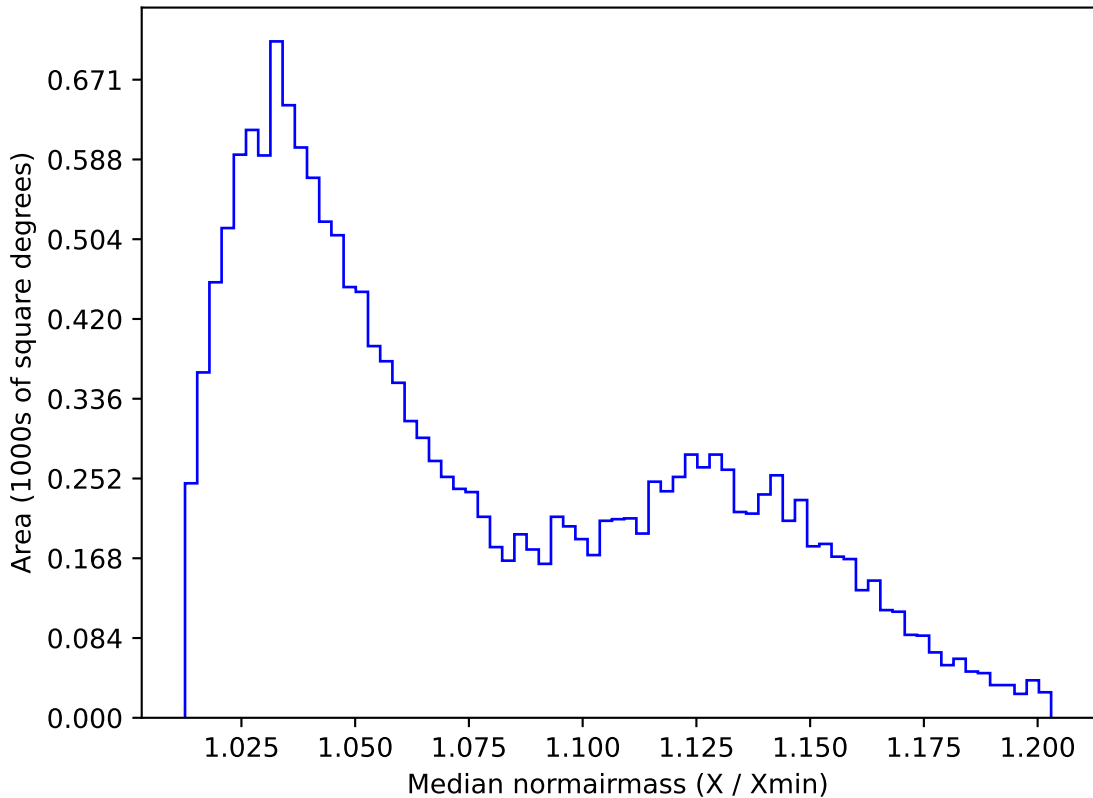
too_elab_r64_d2_ugrizy_v3.4_10yrs WFD u band: Median normairmass
