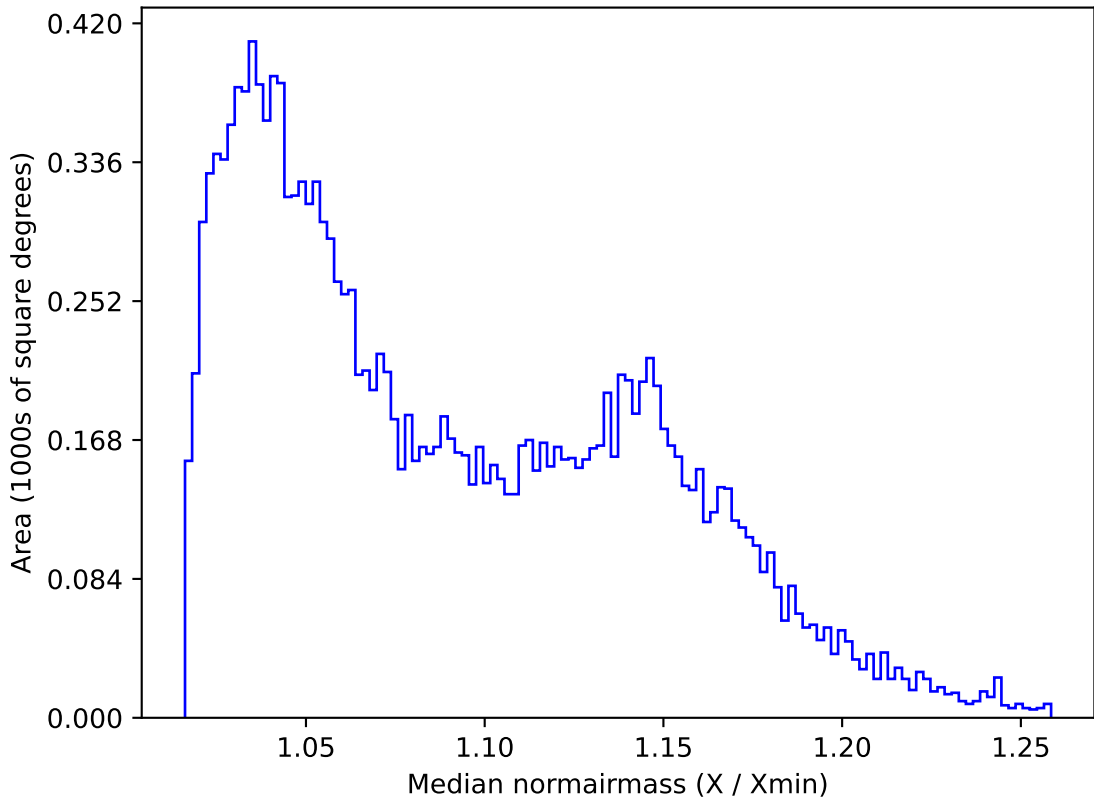
too_elab_r64_d2_ugrizy_v3.4_10yrs WFD g band: Median normairmass
