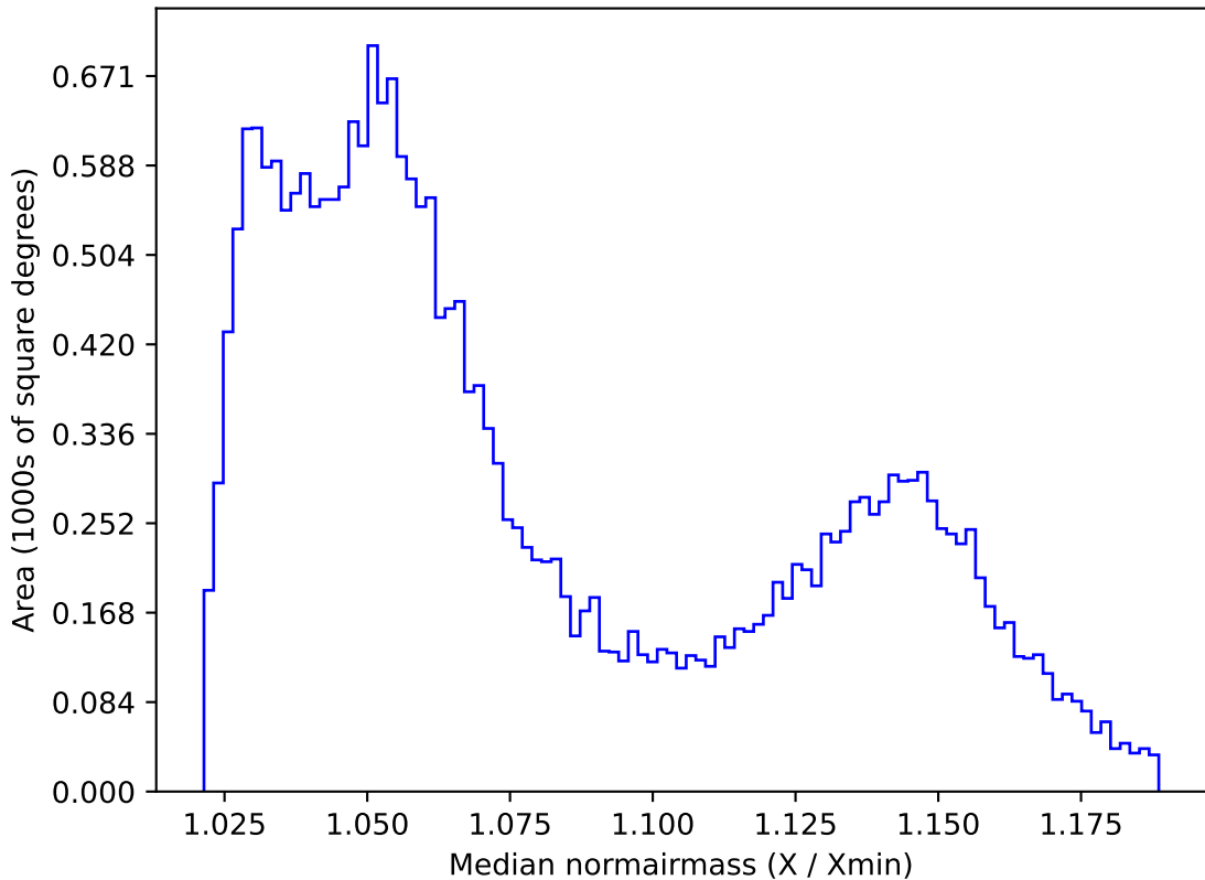
too_elab_r64_d2_ugrizy_v3.4_10yrs All sky all bands: Median normairmass
