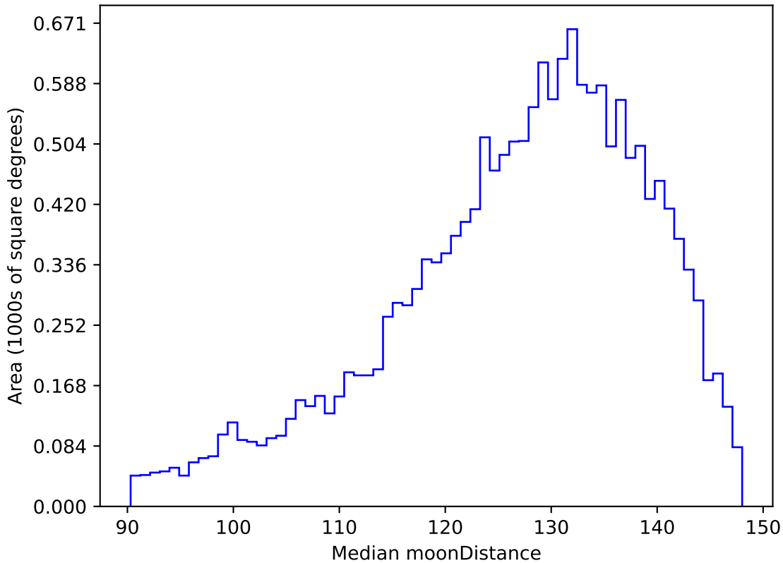
too_elab_r64_d2_ugrizy_v3.4_10yrs WFD u band: Median moonDistance
